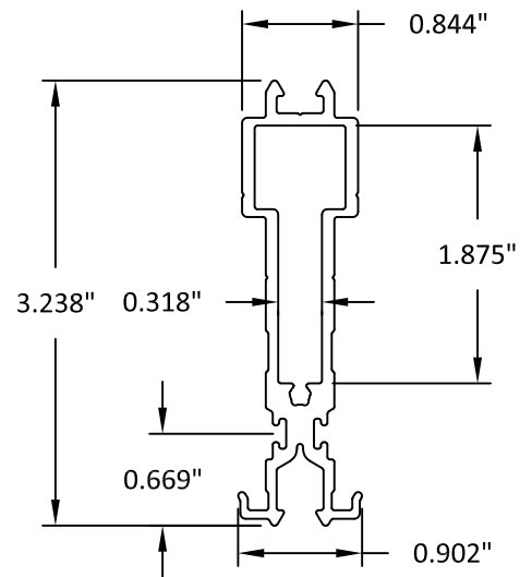
MULLION DETAIL
