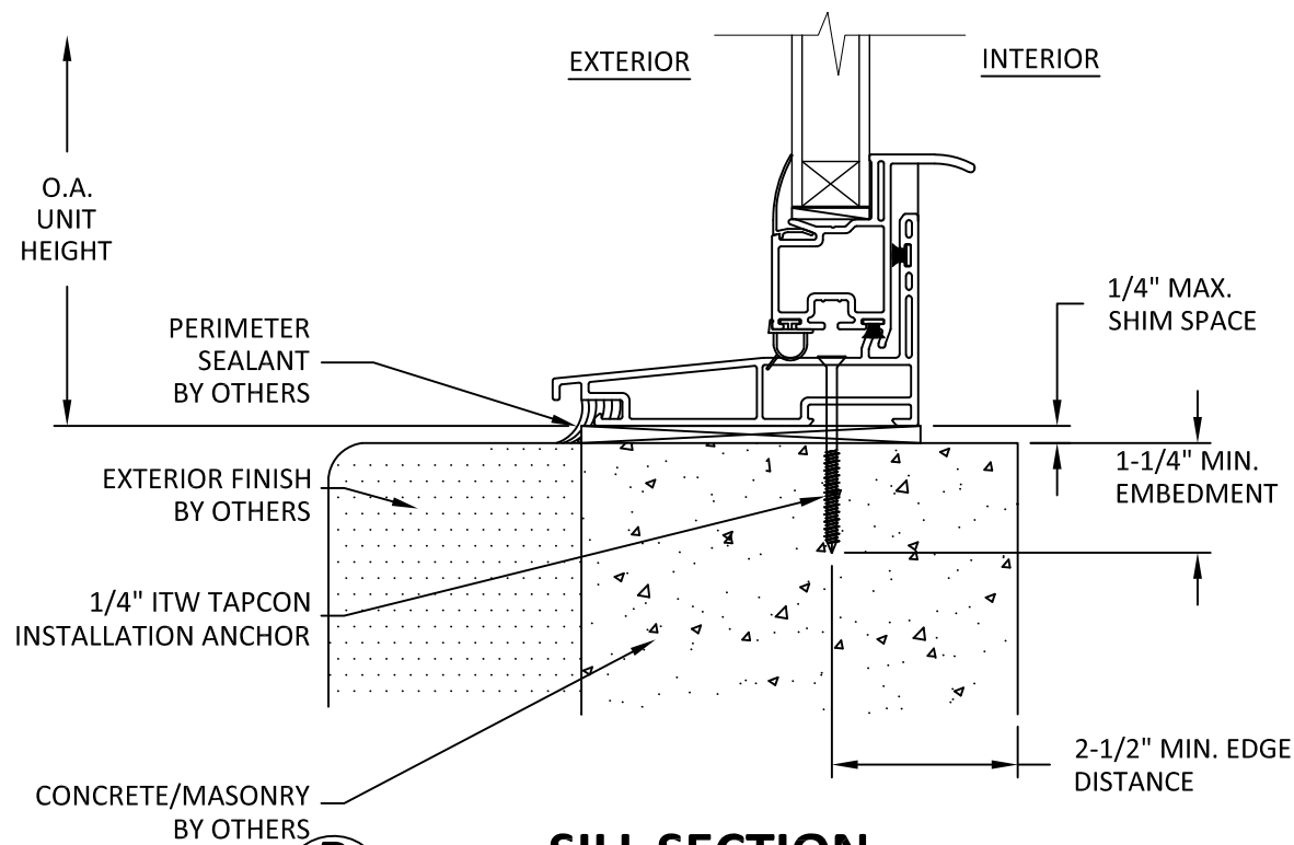
SILL SECTION THROUGH FRAME INSTALLATION (HEAD & SILL ARE INSTALLED THE SAME)
