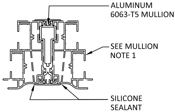
A 2 HORIZONTAL SECTION UNCLIPPED MULLION
