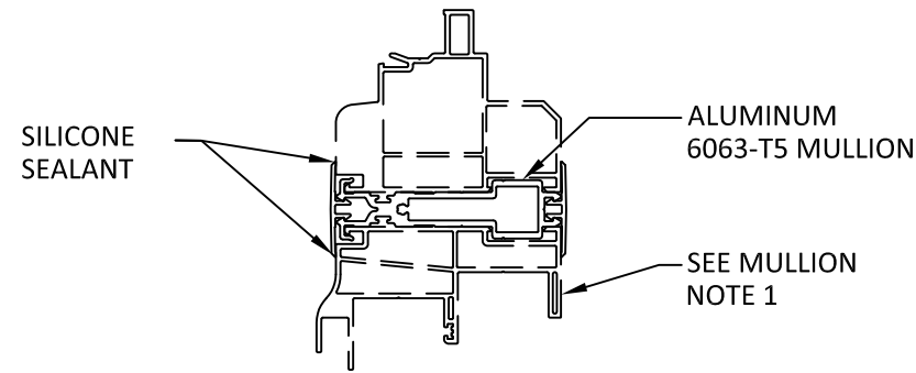
B 2 VERTICAL SECTION UNCLIPPED MULLION
