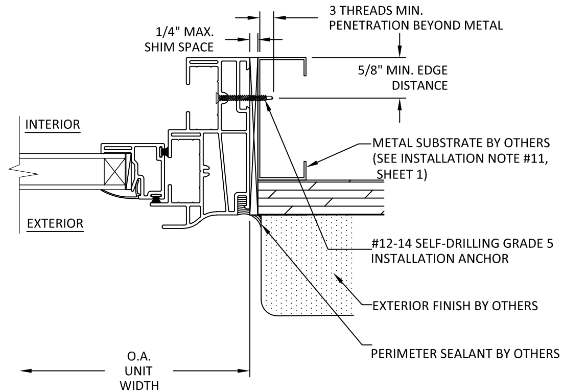
JAMB SECTION THROUGH FRAME INSTALLATION (HEAD & SILL ARE INSTALLED THE SAME)
