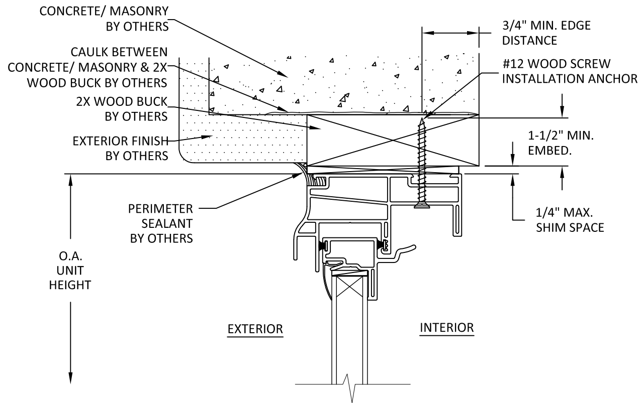
HEAD SECTION THROUGH FRAME INSTALLATION (HEAD & SILL ARE INSTALLED THE SAME)
